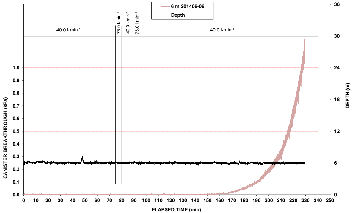
Figure 3-10: CO 2 absorbent canister endurance results; 6 m constant depth
