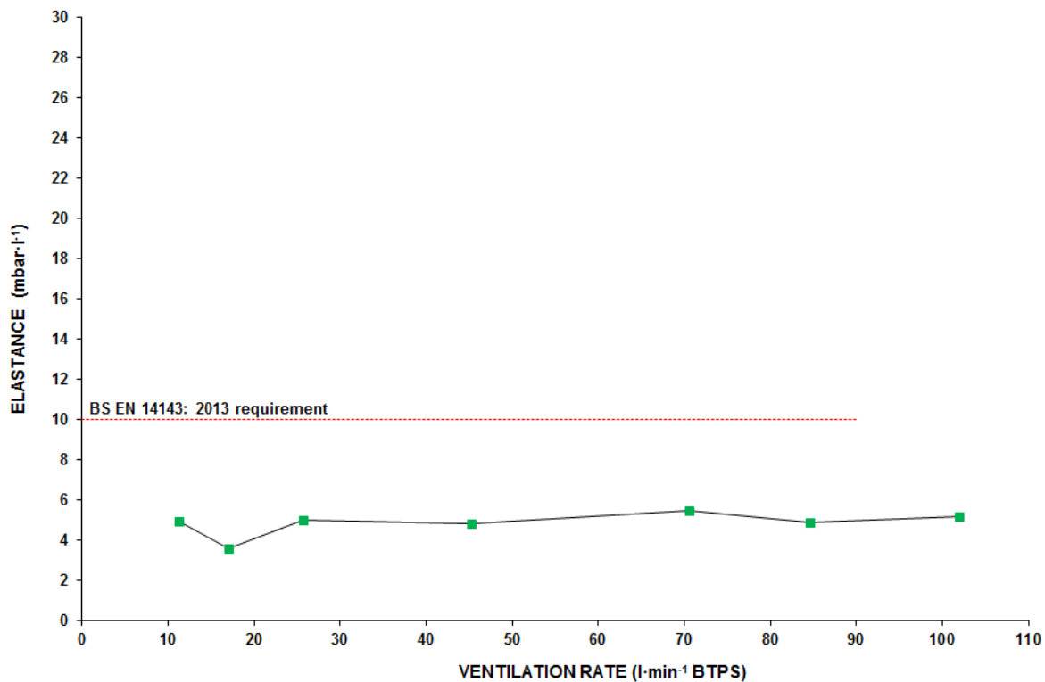
Figure 3-7: Elastance; 100 m, trimix diluent BS EN 14143: 2013 (LSSL reference: 201406-04)
